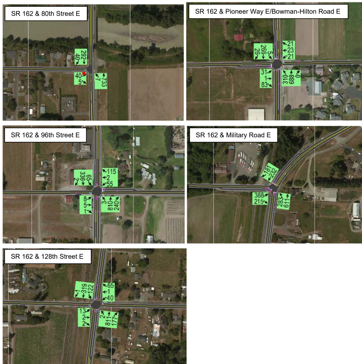
Exhibit 5: P.M. Peak Hour Turning Volumes
