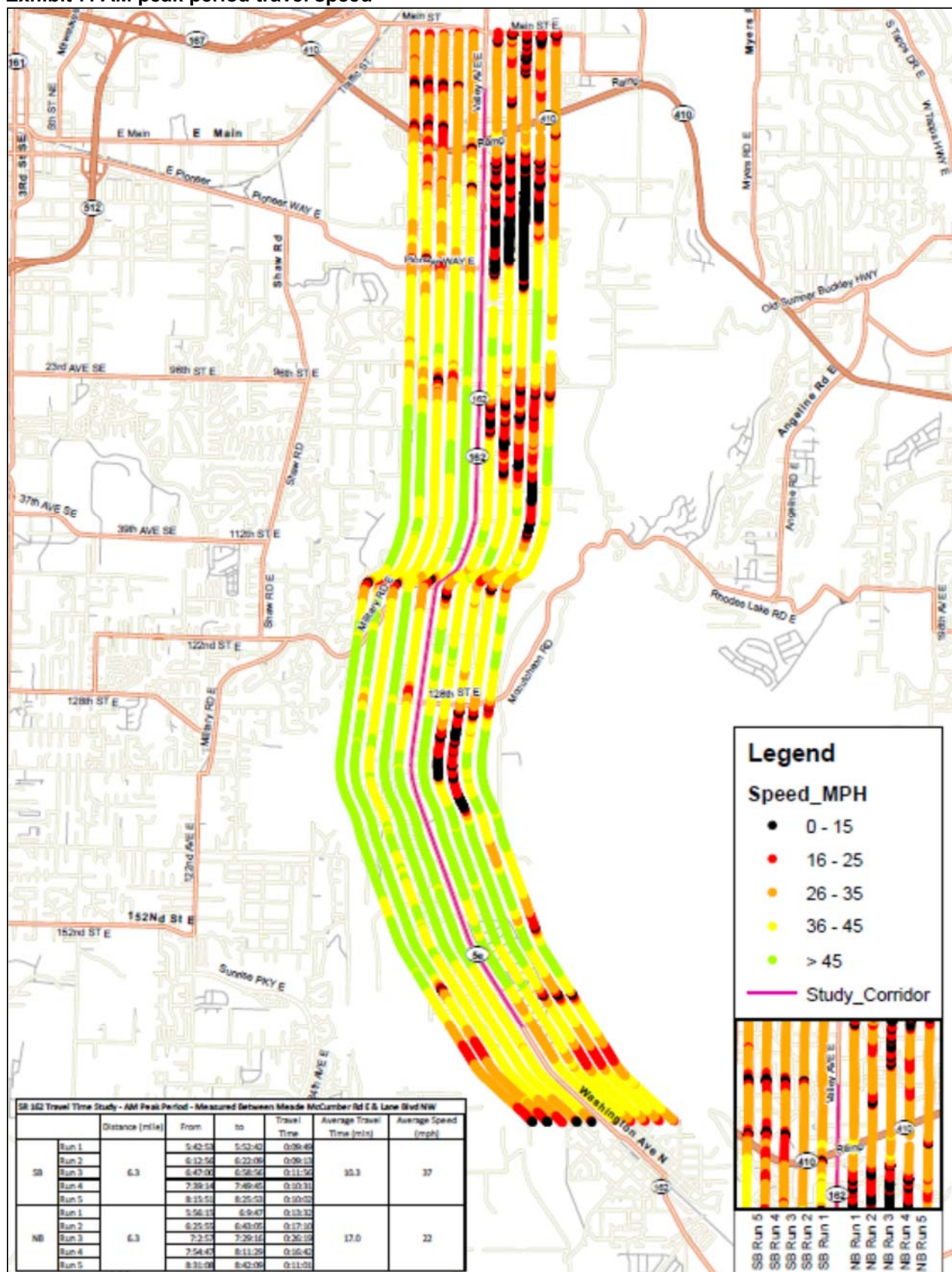
Exhibit 7: AM peak period travel speed
