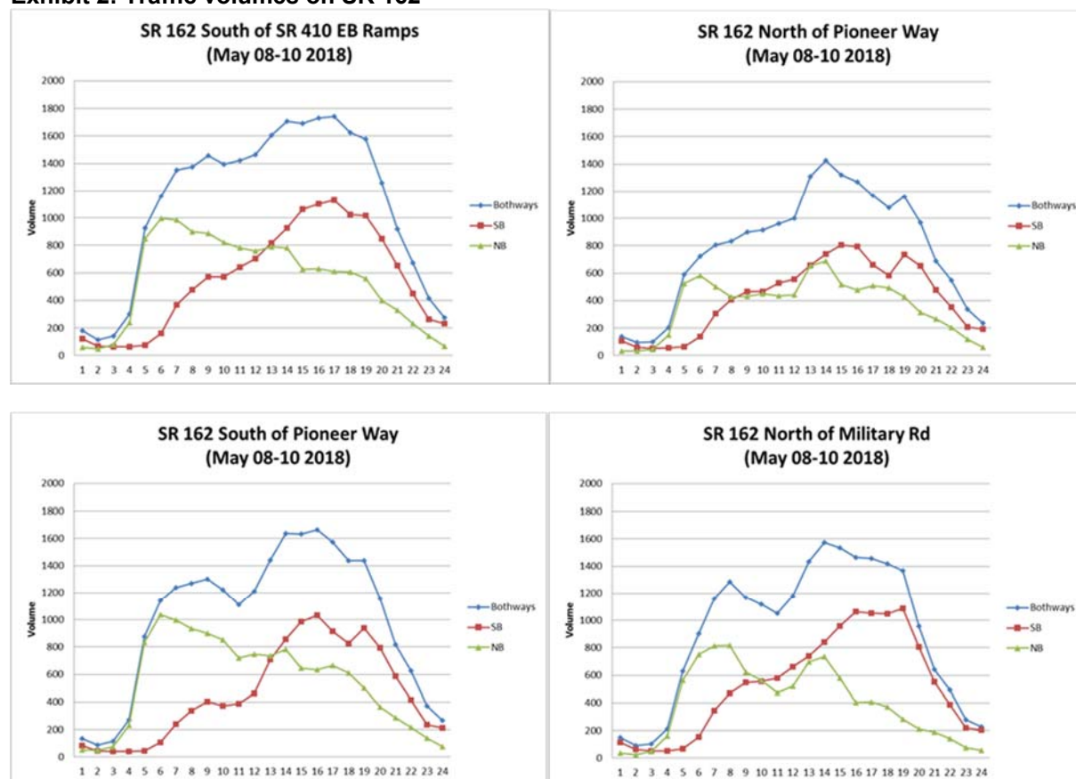
Exhibit 2: Traffic volumes on SR 162
